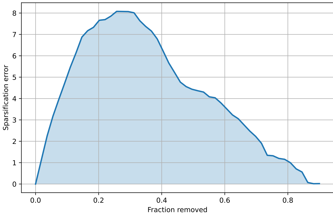
P2P: Sparsification Error Curve AUSE=3.8685 AURG=9.1251
